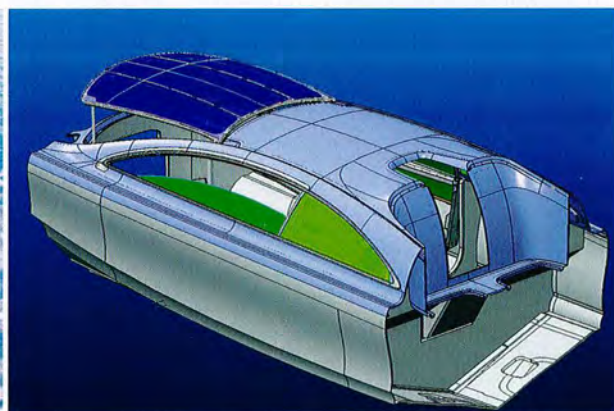
"Arrow 460 Granturismo": Vision Systems of France supplies side windows for this 14-metre Silver Arrows Marine day cruiser, which can be lowered using an electric switch. The large roof window sports an electric dimmer function and can also be raised.
